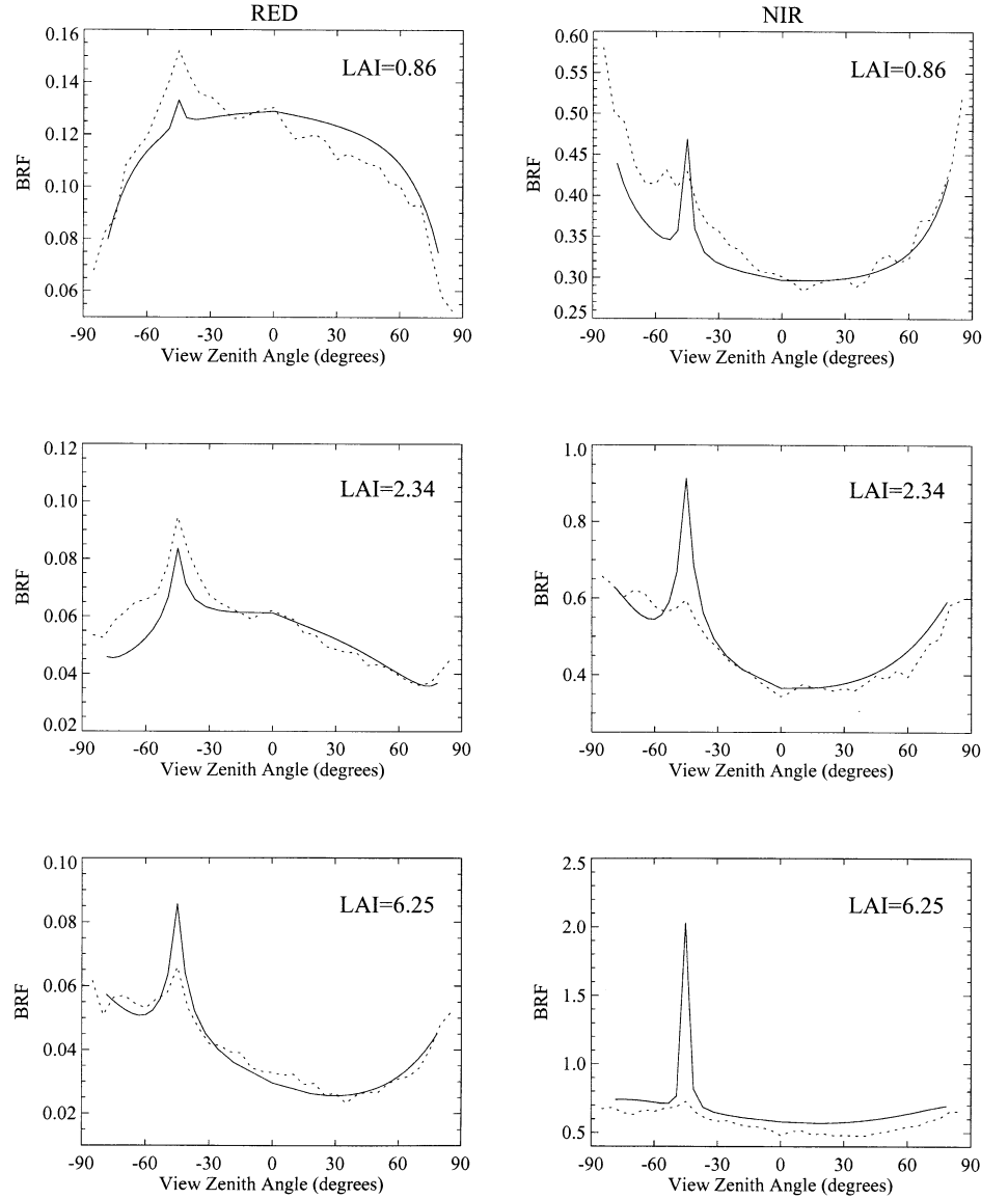
Figure 3. Comparison of BRF in the principal plane simulated by Mean RTE (solid line) and Monte Carlo (dashed line) methods. In all cases soil is “dry,” Cab=50, and SZA=45°.
